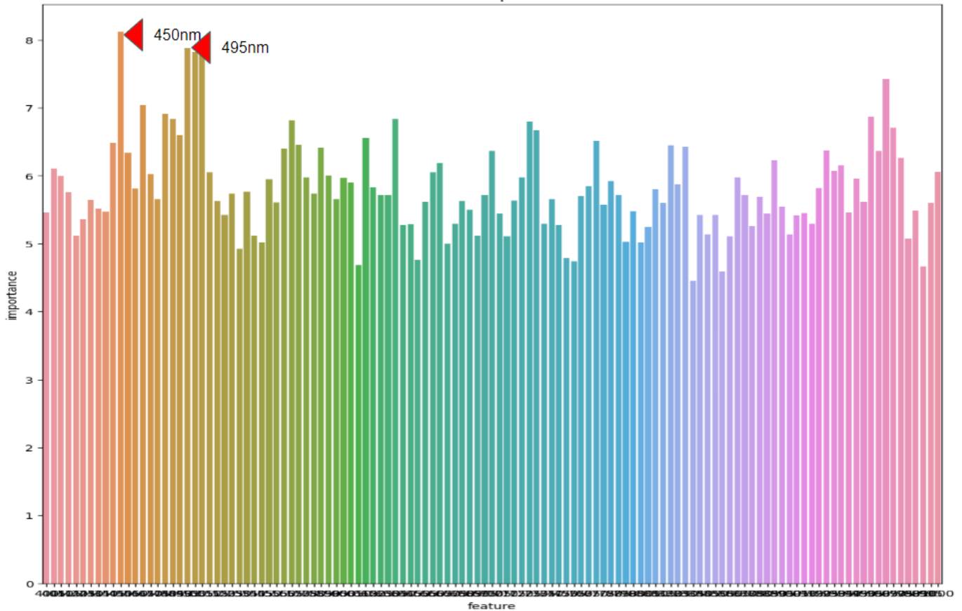
Feature Importance
