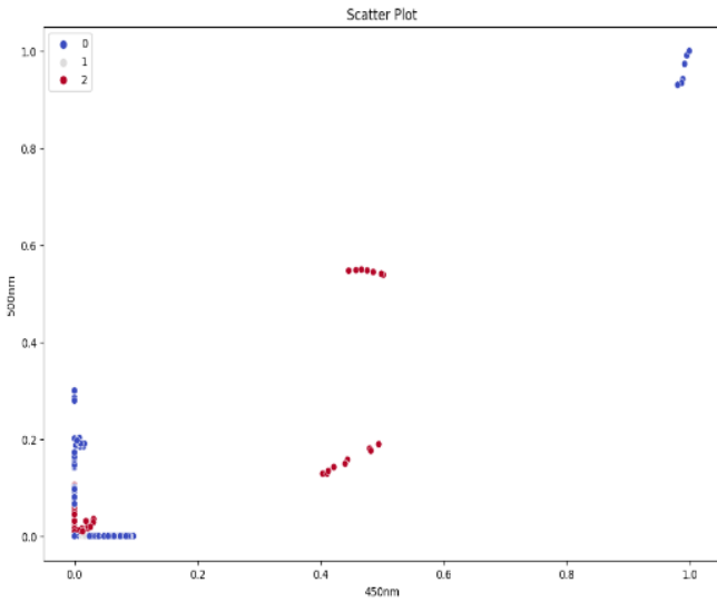
Min-Max Scale
