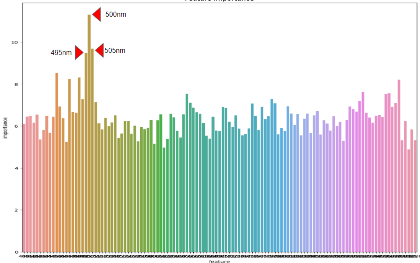
Feature Importance
